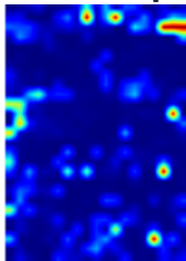
attention
